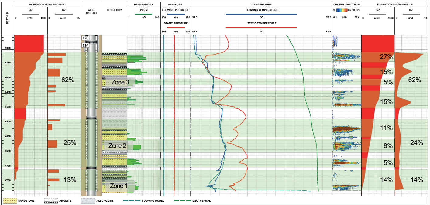
Example 1. Accurate flow diagnostics for a horizontal gas well used to optimise development of a low-permeability reservoir Horizontal Flow diagnostics with Cascade3 delivered an accurate gas production profile in a horizontal well drilled in a low-permeability, gas-bearing formation. The well was completed using a slotted liner across three zones separated by swellable packers. The contribution of each active permeable unit was accurately quantified with a continuous flow profile. The survey defined production contributions from each of the reservoir subunits, thereby improving the hydrodynamic reservoir model and making it possible to optimise subsequent wells in the ongoing field-development programme.
