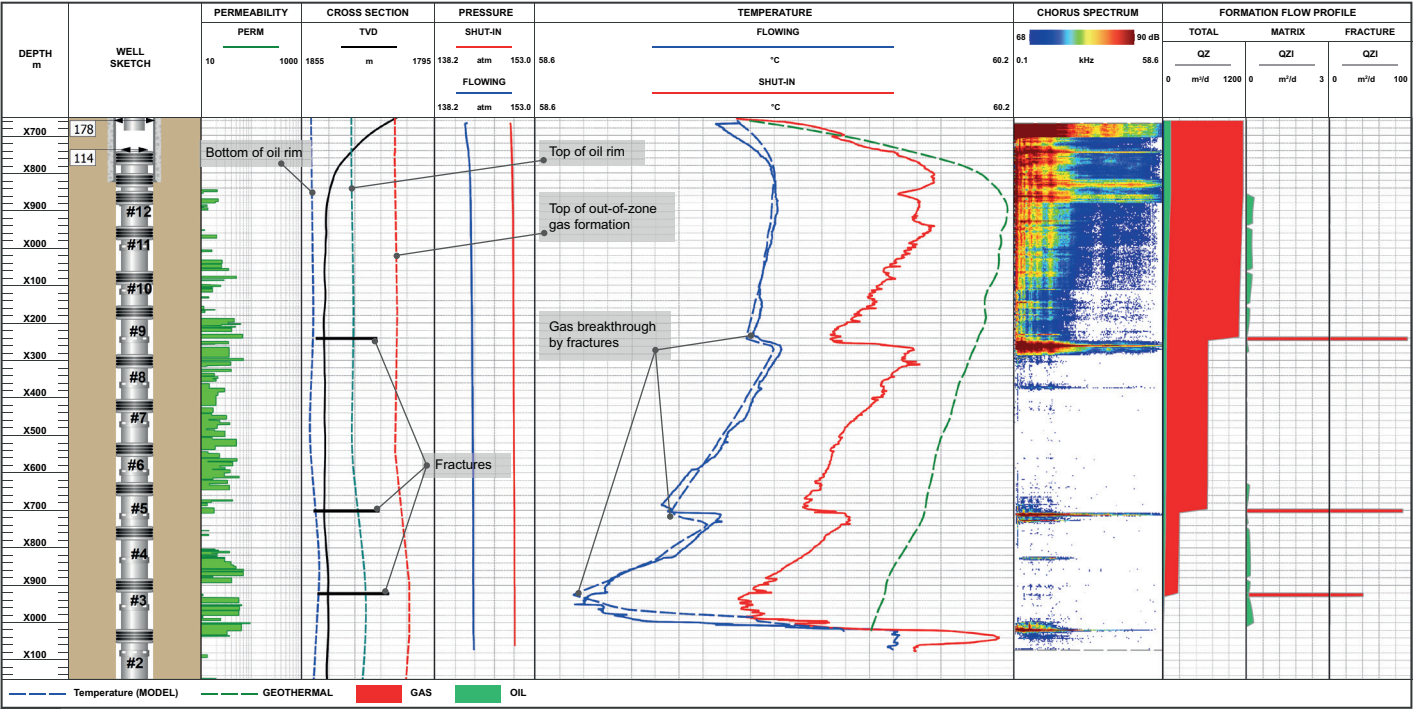
Example 2. Identifying gas breakthrough in a horizontal oil producer with multistage fractures helps to optimise fracture design The Horizontal Flow survey identified three gas breakthrough zones responsible for the well's high gas/oil ratio, and estimated potential fracture growth, thereby indicating how far the fractures penetrated into the overlying gas-bearing formation. Fracture entry points behind the liner were assessed using the Chorus platform. This also revealed fractures in the target oil-bearing formation that were idle or nonproductive owing to the gas breakthrough. For future wells, the operator has redesigned the fracture programme so that production from the low-permeability oil rim can be maximised while preventing gas breakthroughs caused by out-of-zone fractures.
